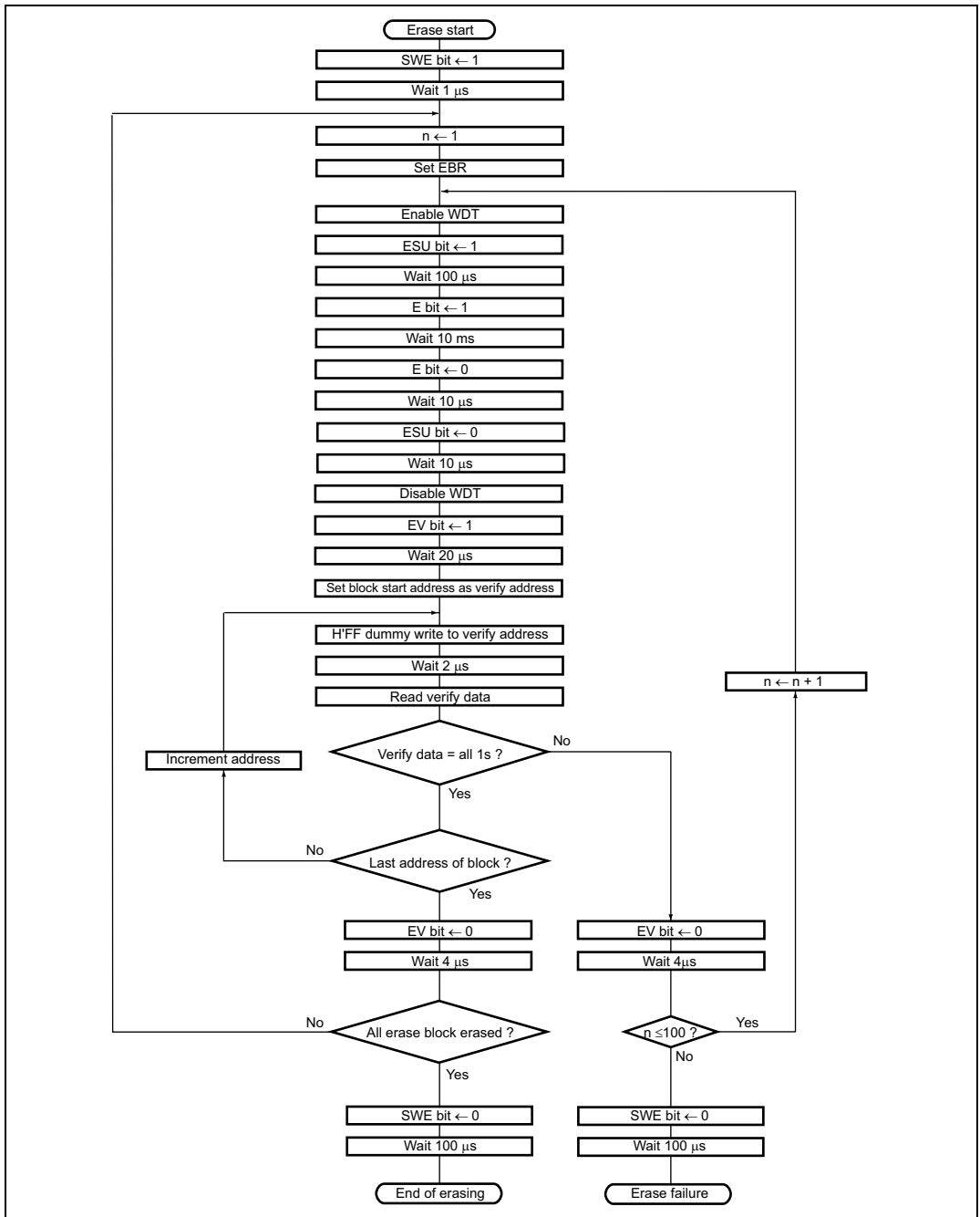
Figure 6.11 Erase/Eraser-Verify Flowchart
