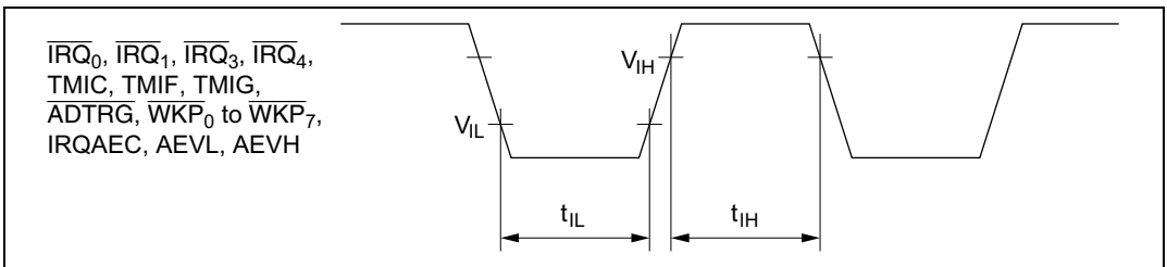
Figure 16.3 Input Timing
